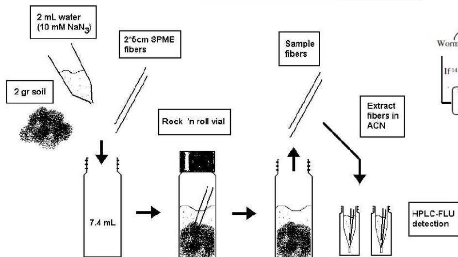
Figure 1: A schematic picture of negligible depletion passive samplers to measure freely dissolved aqueous concentrations of contaminants in soil.
