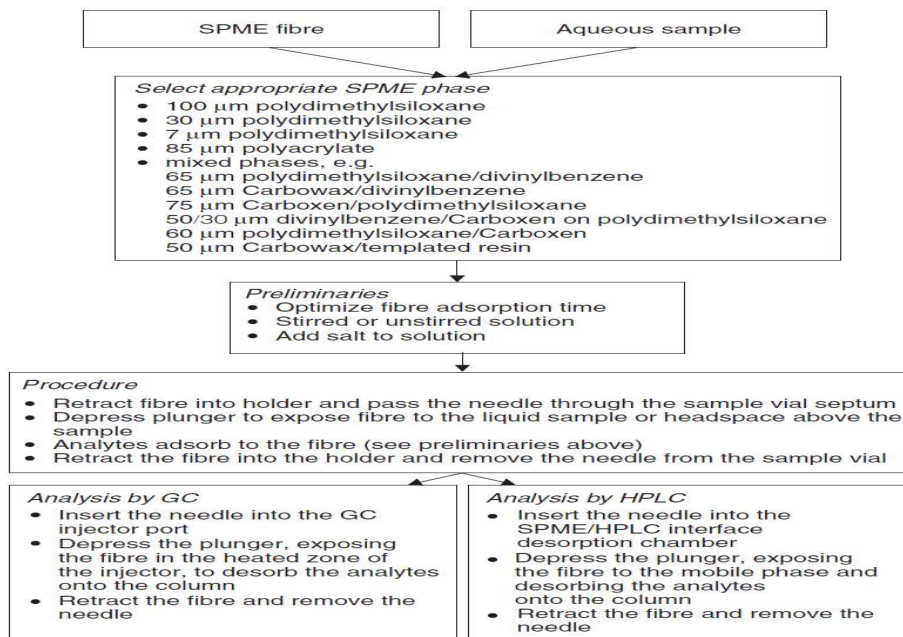
Figure 3.10 Typical procedure used for the solid-phase microextraction of liquids. From Dean, J. R., Methods for Environmental Trace Analysis , AnTS Series. Copyright 2003. © John Wiley & Sons, Limited. Reproduced with permission.
