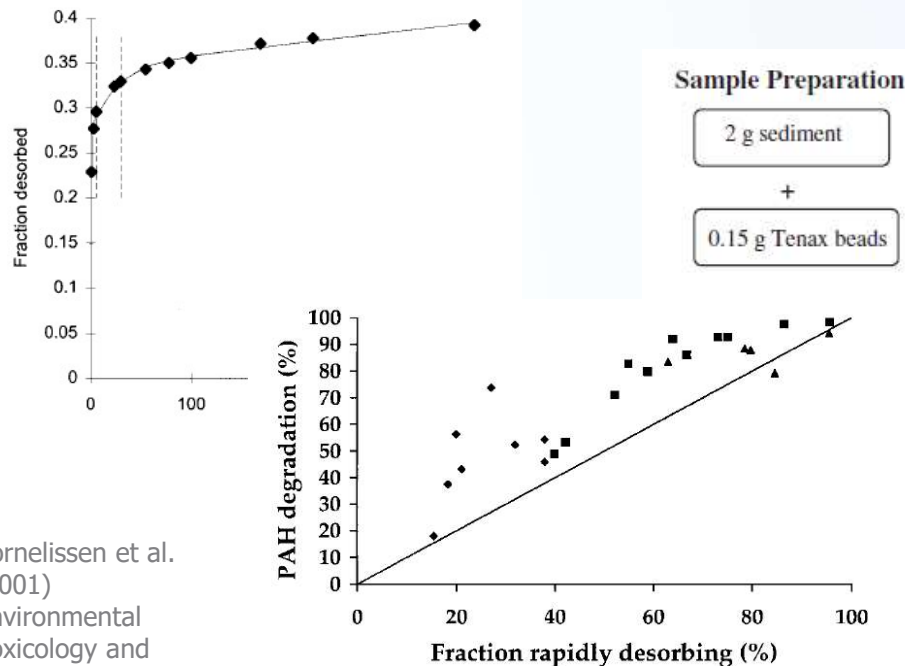
Fig. 3. Estimation of polycyclic aromatic hydrocarbon (PAH) bioavailability using Tenax. Amount degraded (%) versus rapidly desorbed (%). Degradation in a bioreactor (■ and ▲) or by landfarming (◆) (Cornelissen et al., 1998a, b).
