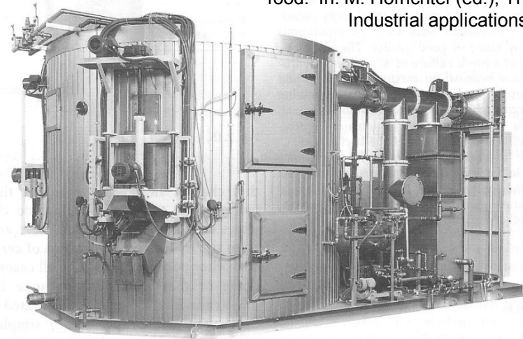
Fig. 2.13. Rotary type automatic koji making equipment. Reproduced with permission from Fujiwara Techno-Art Co. Ltd., Japan
