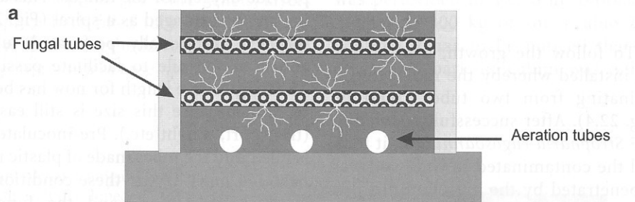
Fig. 22.6. Spiral aeration system of a fungal pilot pile. It can be connected to a compressor for continuous active aeration
