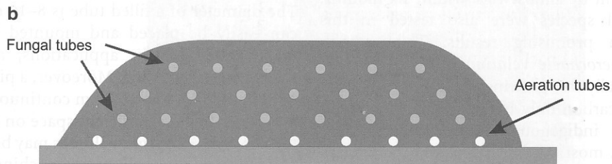
Fig. 22.7. Schematic cross-sections through a pile based on fungal tube technology
