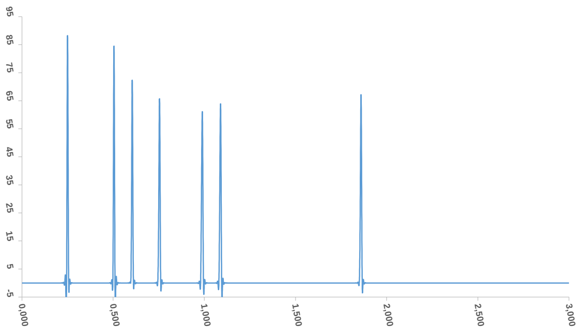
Simulated gradient elution, V_D = 0 ml
