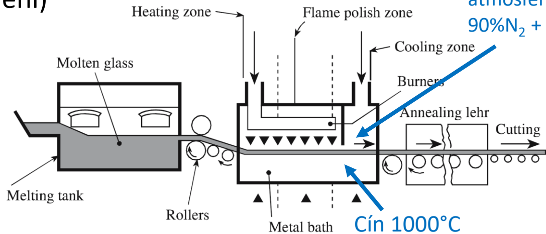
FIGURE 26.9 Schematic diagram of the float glass process.
