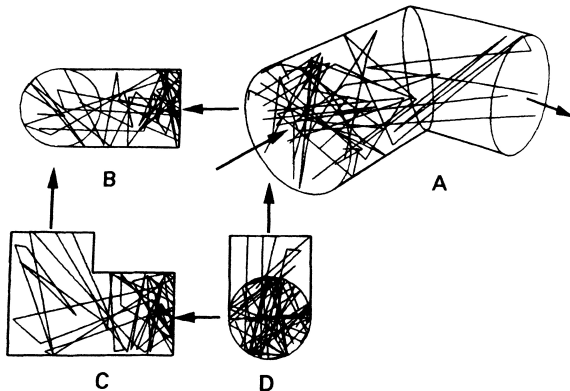
Fig. 3.4 A computer graphical display of the trajectories of 15 molecules entering an elbow in free molecular flow. Courtesy of A. Appel, IBM T. J. Watson Research Center.
