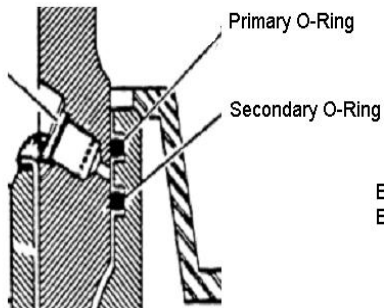
Detail: O-Ring Cross-Section
