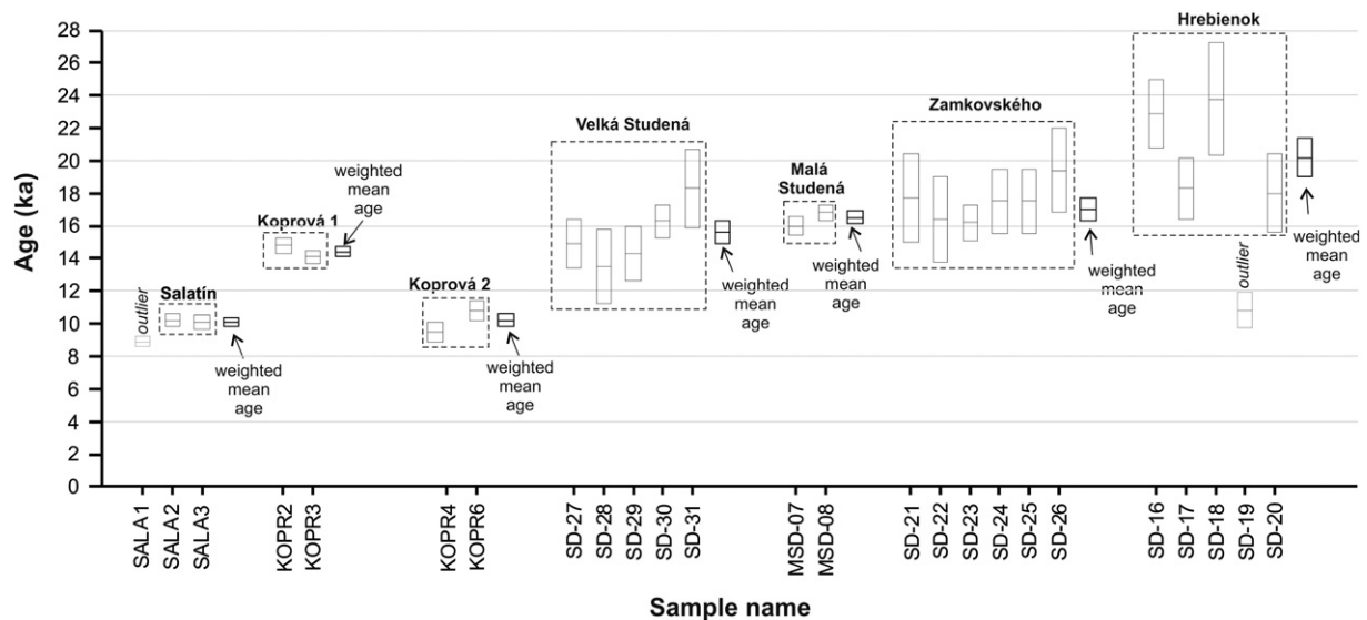
Fig. 7. ^{10}\text{Be} and weighted arithmetic mean dates for studied RSFs. Arithmetic means are plotted to the right of the data block for each RSF. Statistical outliers were not used in weighted mean age calculations and are marked in grey.
