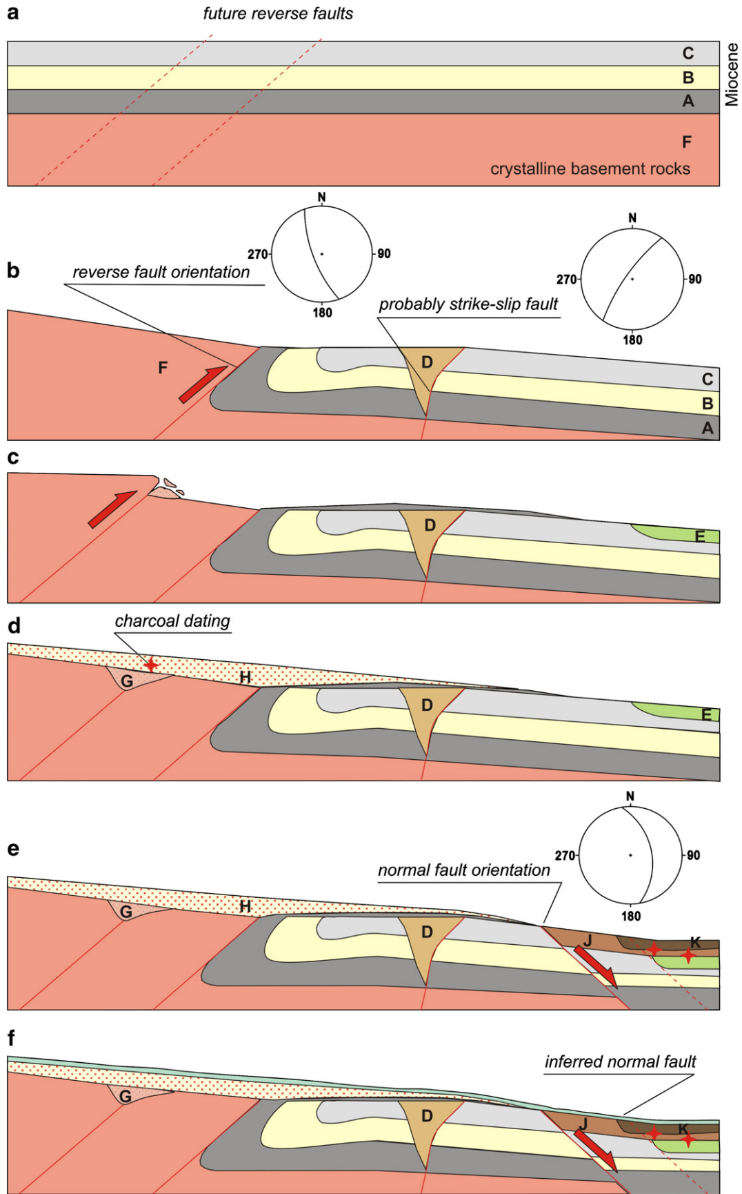
Fig. 11. Retro-deformation series of movements interpreted from the Trench P2. a) initial position of Miocene fluvial to limnic sediment layers (A–C) overlaying crystalline basement (F), b) reverse faulting that dragged Miocene layers and strike-slip movements cutting the sediments, followed by erosion, c) younger reverse faulting that follows deposition of Late Pleistocene alluvial fan (E) and gelification of Miocene layers, d) fault scarp erosion and deposition of colluvial wedge (G) followed by deposition of early Holocene colluvial sediments (H), e) (?) normal faulting and possibly related deposition of Member J, followed by deposition of the youngest colluvial sediments (K), and f) present-day situation with recent topsoil.
