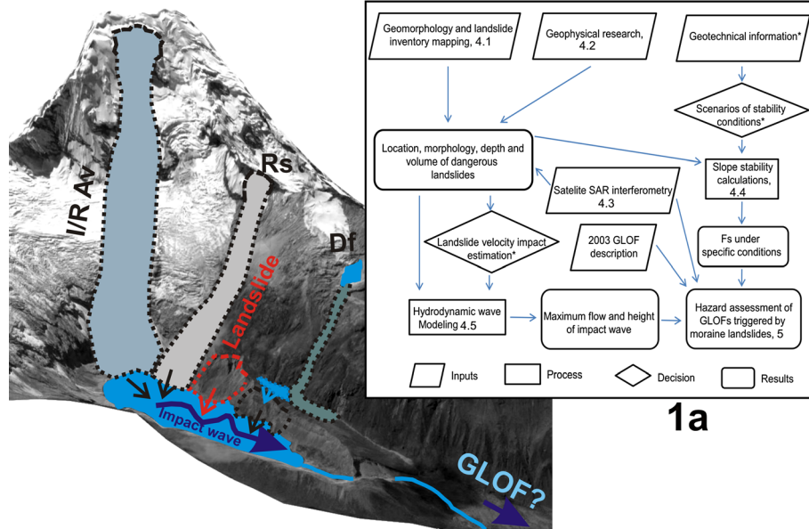
Fig. 1 Schematic diagram showing theoretical types of slope processes which could triggered GLOFs in the Cordillera Blanca Mts., Peru, representing only fraction of all possible GLOF initiation processes (Emmer and Cochachin 2013; Richardson and Reynolds 2000). Ice/rock avalanche ( I/R Av ) caused the 2010 GLOF from Lake 513 (Klimeš et al. 2014; Schneider et al. 2014); rockslide ( Rs ) initiated the 2002 GLOF from Safuna Alta Lake (Hubbard et al. 2005); landslide from lateral moraine caused the 1953 GLOF from Tullparaju Lake (Lliboutry et al. 1977a), the 2003 GLOF from Palcacocha Lake (Vilímek et al. 2005), and the 2012 GLOF from Artizon Alto Lake (Emmer et al. 2014); a debris flow ( Df ) from a valley dammed temporal lake, which initiated a landslide from the inner slope of the Cangrajanca Lake lateral moraine (Cordillera Huayhuash, Peru, Engel et al. 2011). a Workflow diagram showing the steps taken to achieve complex knowledge of processes and conditions affecting hazard imposed by GLOFs triggered by landslides originating in the lateral moraines of the Palcacocha Lake. Asterisks indicate steps where review of available literature was extensively used. Ch. chapter, Fs factor of safety
