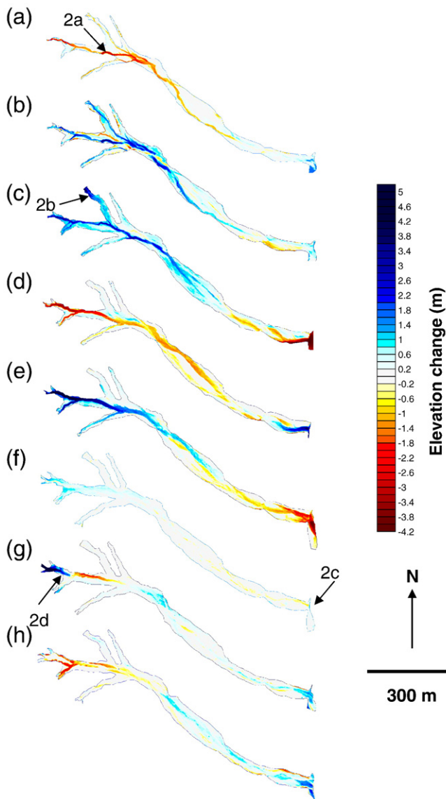
Fig. 5. DEMs of difference for successive surveys: (a) December 2004–April 2005, (b) April 2005–August 2005, (c) August 2005–December 2005, (d) December 2005–May 2006, (e) May 2006–August 2006, (f) August 2006–November 2006, (g) November 2006–April 2007, (h) April 2007–August 2007. Numbers indicate location of photos in subsequent figures (Fig. 6).
