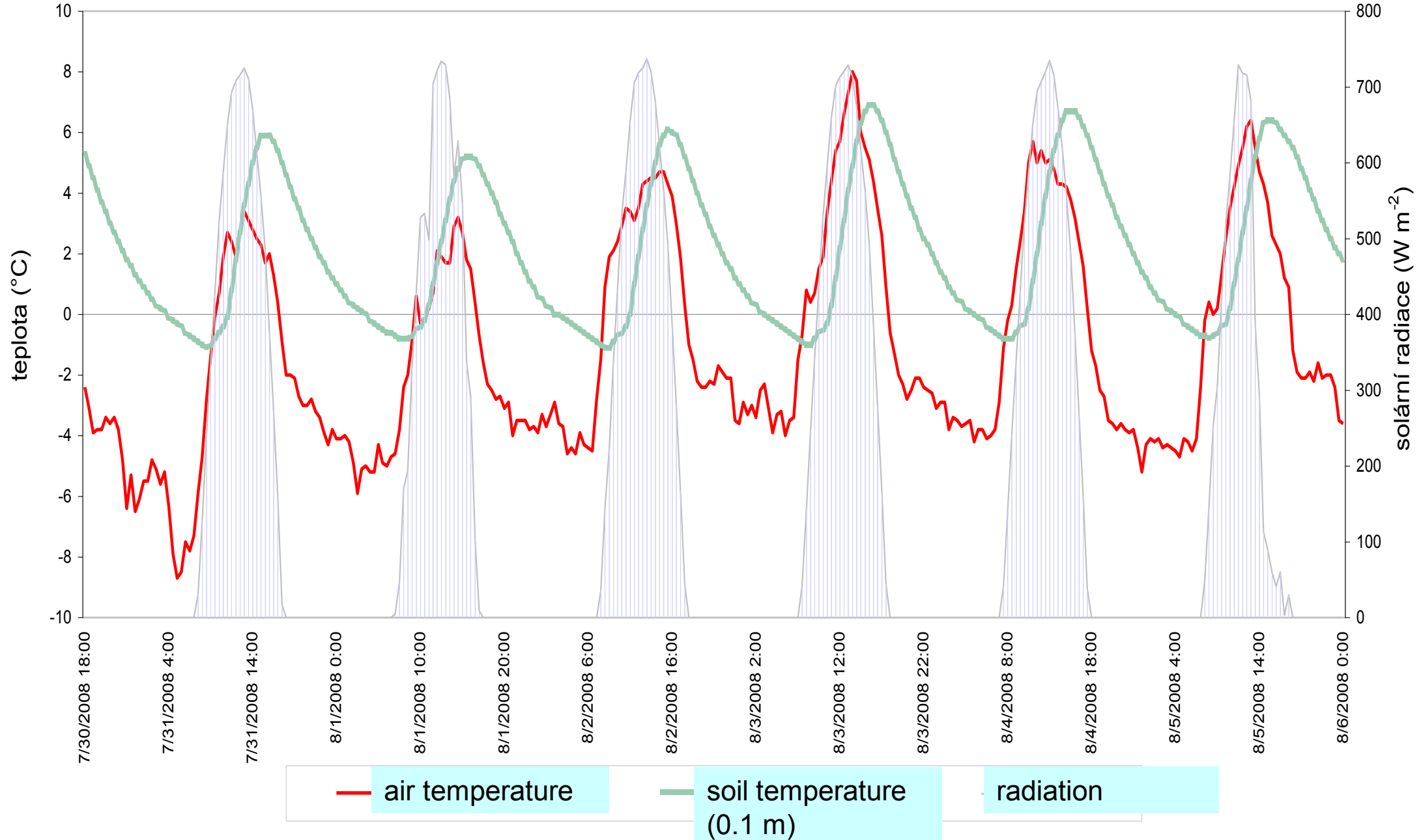
Air temperature, soil temperature and solar radiation at the Amazon's source. The climatic station of the Charles University in Prague (5075 m a.m.s.l., period 30.7. - 6.8. 2008).
