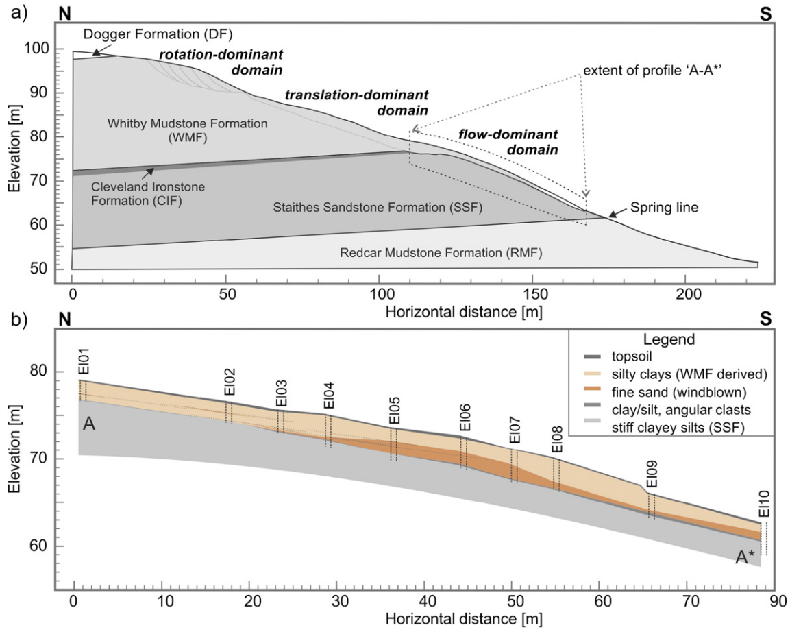
Fig. 2. Representative section of the stratigraphy and slope instability domains for Hollin Hill. a) Diagram modified after Gunn et al. (2013). b) Profile A-A* through the eastern lobe informed by hand augered holes down to depth of 4 m (profile location indicated in Fig. 1).
