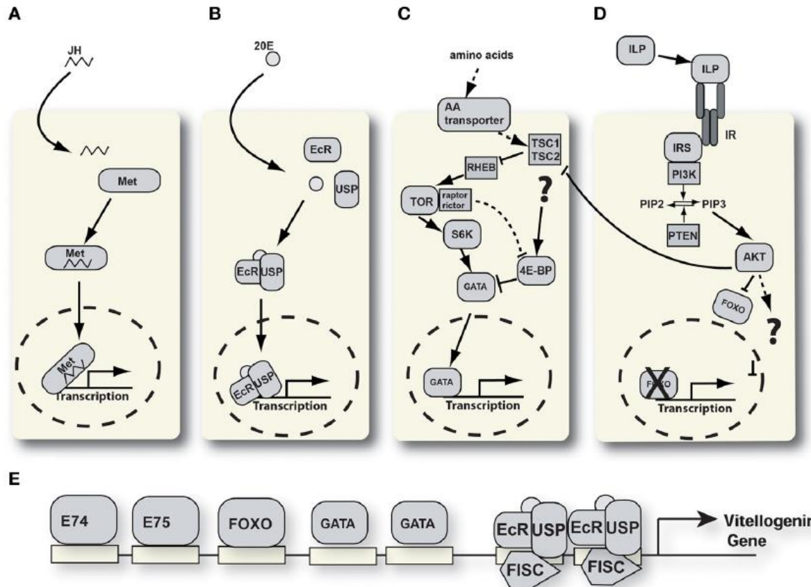
FIGURE 2 | Signaling pathways involved in YPP regulation. (A) Juvenile hormone signaling pathway. JH, juvenile hormone; Met, methoprene tolerant. (B) Ecdysone signaling pathway. 20E, 20 hydroxyecdysone; EcR, ecdysone receptor; USP, ultraspiracle. (C) Nutrient signaling pathway. 4E-BP, 4E-binding protein; TSC, tuberous sclerosis complex; RHEB, RAS homologue enriched in brain; S6K, S6 kinase; TOR, target of rapamycin. (D) Insulin-like
