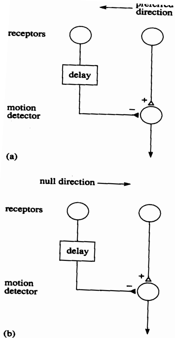
Figure 4.36 Principles of a simple retinal motion detector. See text for explanation.
