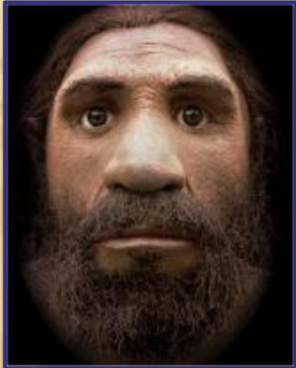
Homo neanderthalensis
