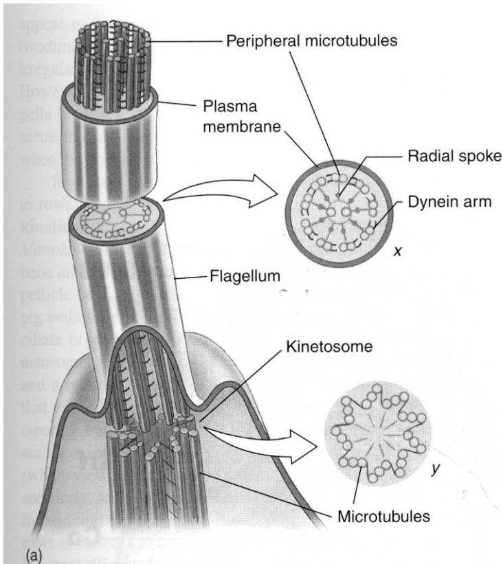
Figure 4.4 Flagella (undulipodia).
