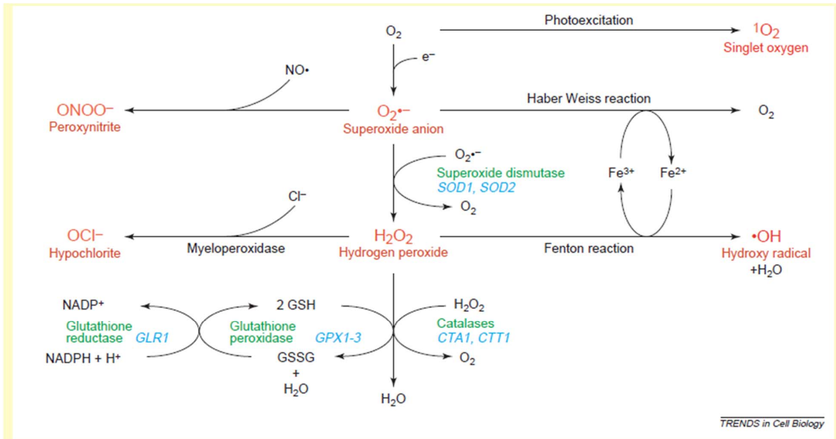
Figure I. ROS and other radicals generated in cells. Reactive intermediates are in red, key antioxidant enzymes are in green and the genes that encode them in yeast are in blue. Myeloperoxidase is produced by neutrophils as part of the cellular defense system against microorganisms.
