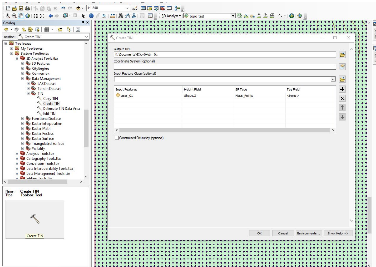
Obr. 8 Create TIN
