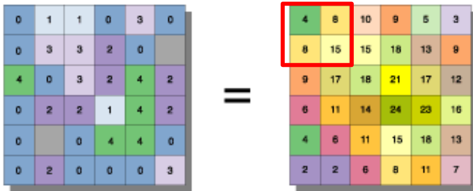
The Neighborhood Function on a Grid
