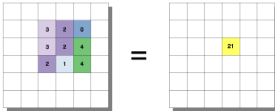
The Neighborhood Function on an Individual Neighborhood
