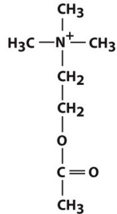
(A) acetylcholine
