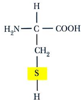
CYSTEINE
