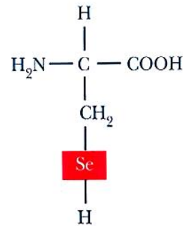
SELENOCYSTEINE
