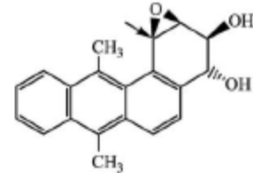
3S,4R,1R,2S-DMBA-diol epoxide
