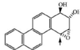
1R,2S,3S,4R-CHR-diol epoxide
