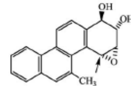
1R,2S,3S,4R-5MC-diol epoxide
