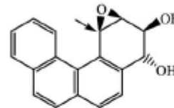
3S,4R,1R,2S-BcPh-diol epoxide
