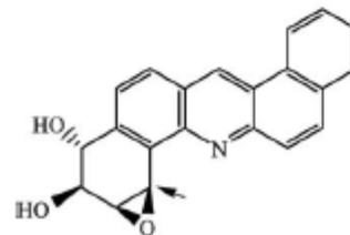
10S,11R,8R,9S-DB[a,h]A-diol epoxide
