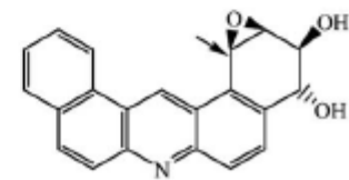
3S,4R,1R,2S-DB[a,j]A-diol epoxide
