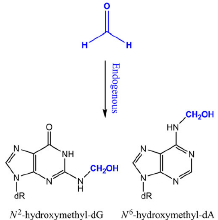
Steady-State Amounts of Selected endogenous DNA Damage
