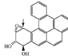
11R,12S,13S,14R-DB[a,l]P-diol epoxide
