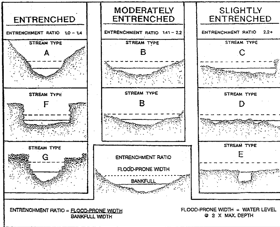
Fig. 6. Examples and calculations of channel entrenchment.
