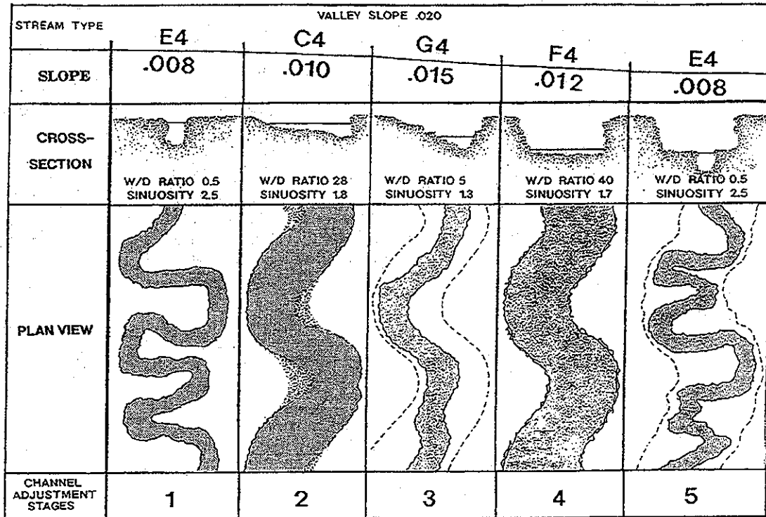
Fig. 9. Evolutionary stages of channel adjustment.
