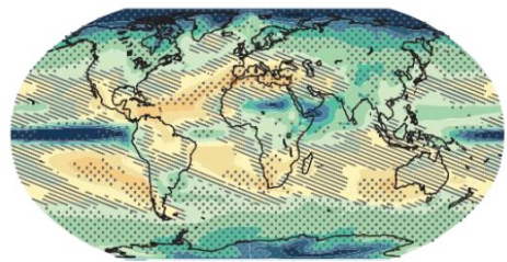
RCP 8.5
