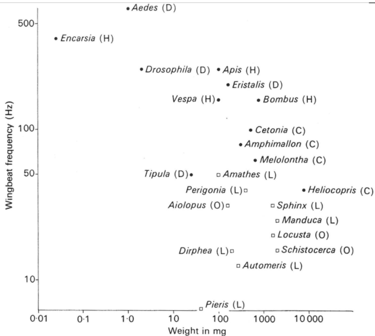
Fig. 138 Relationship between wingbeat frequency and weight in various insects. □— insects with synchronous muscles, ●—insects with asynchronous muscles. C—Coleoptera, D—Diptera, H—Hymenoptera, L—Lepidoptera, O—Orthoptera (mainly after Weis-Fogh, 1973; Bartholomew and Casey, 1978)
