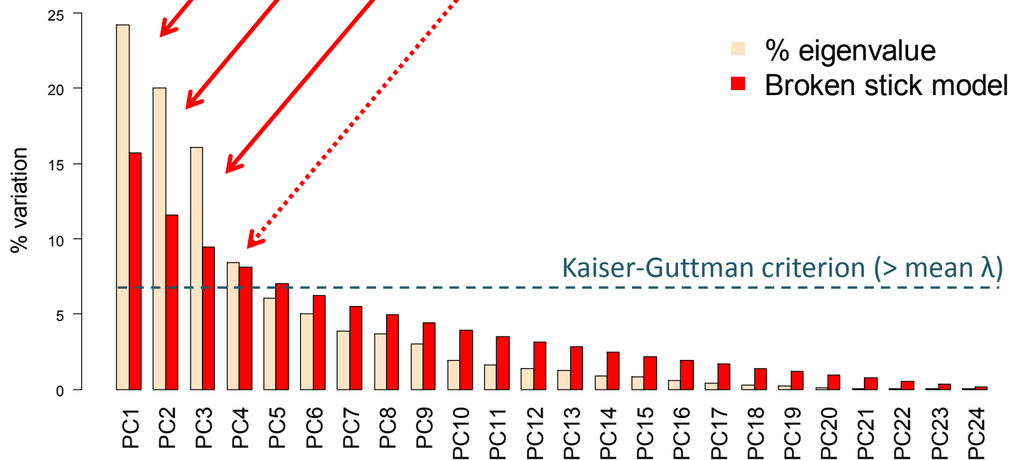
Screeplot
