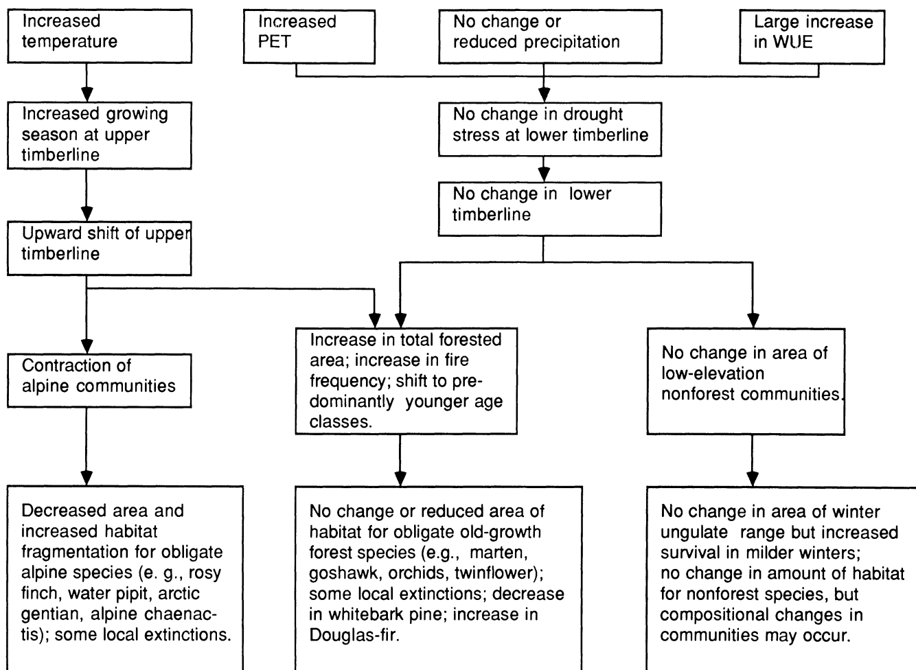
Figure 3. Potential effects on the Greater Yellowstone Ecosystem of a climate that is warmer and drier than the present climate, but with a compensating increase in plant water use efficiency (scenario 2).
