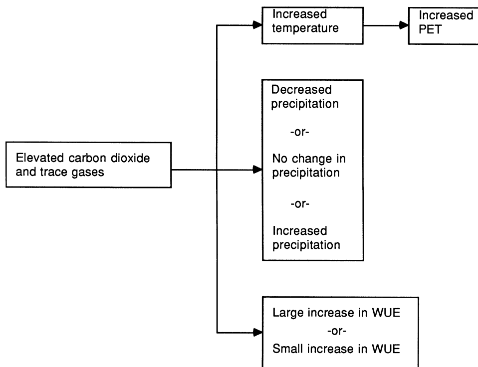
Figure 1. Potential effects of projected climate change in the Greater Yellowstone Ecosystem. PET = potential evapotranspiration; WUE = plant water use efficiency.
