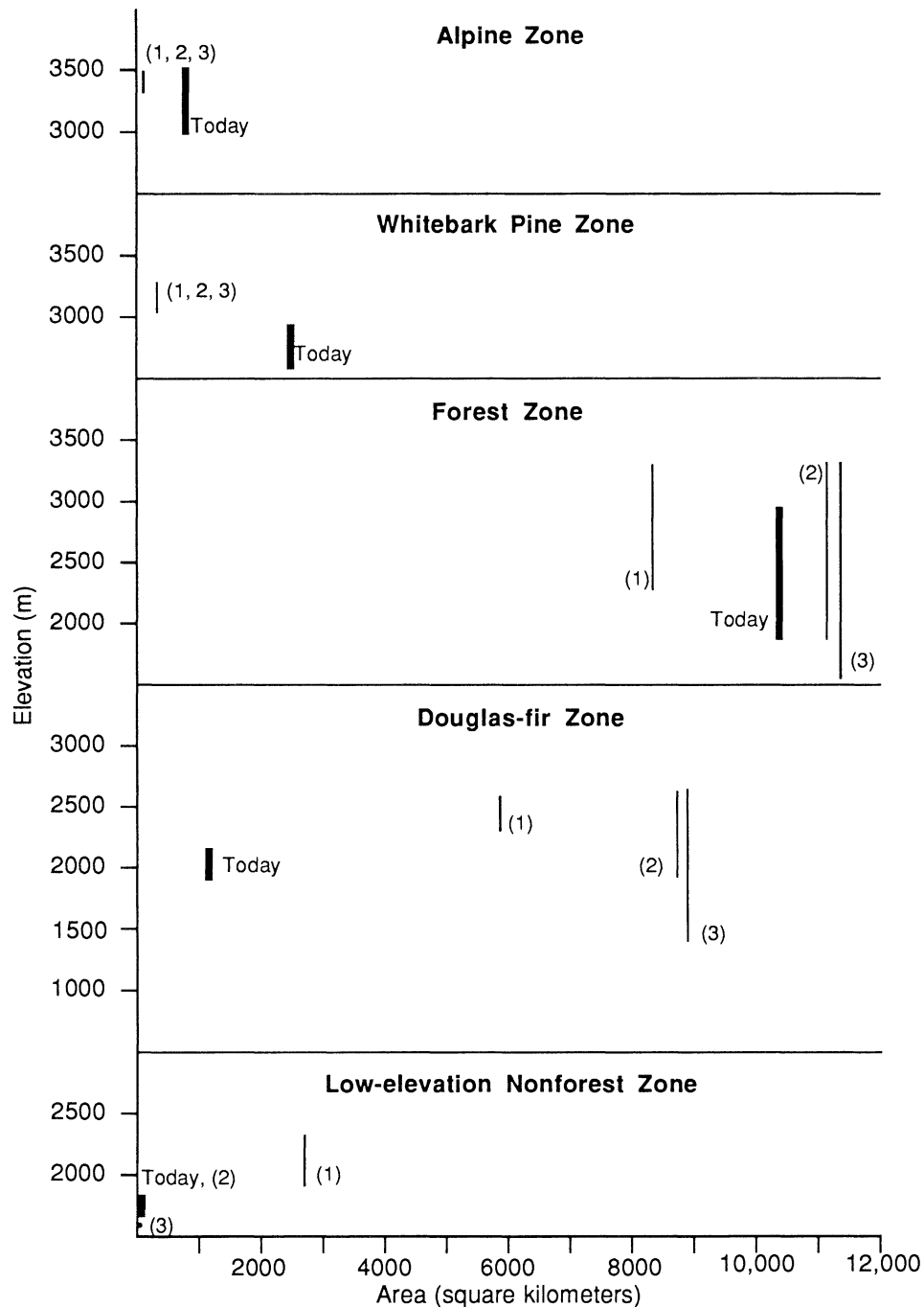
Figure 6. Present and projected areas and elevational ranges of vegetation zones in Yellowstone National Park and the adjacent mountains along its eastern border. Scenario (1) is elevated temperature, CO_2 , and drought stress. Scenario (2) is elevated temperature, but no change in drought stress. Scenario (3) is elevated temperature and CO_2 , but reduced drought stress. See text for details.
