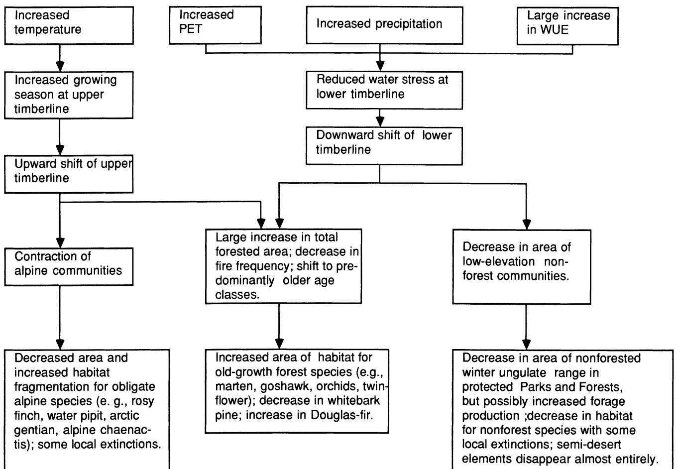
Figure 4. Potential effects on the Greater Yellowstone Ecosystem of a climate that is warmer and wetter than the present climate (scenario 3).
