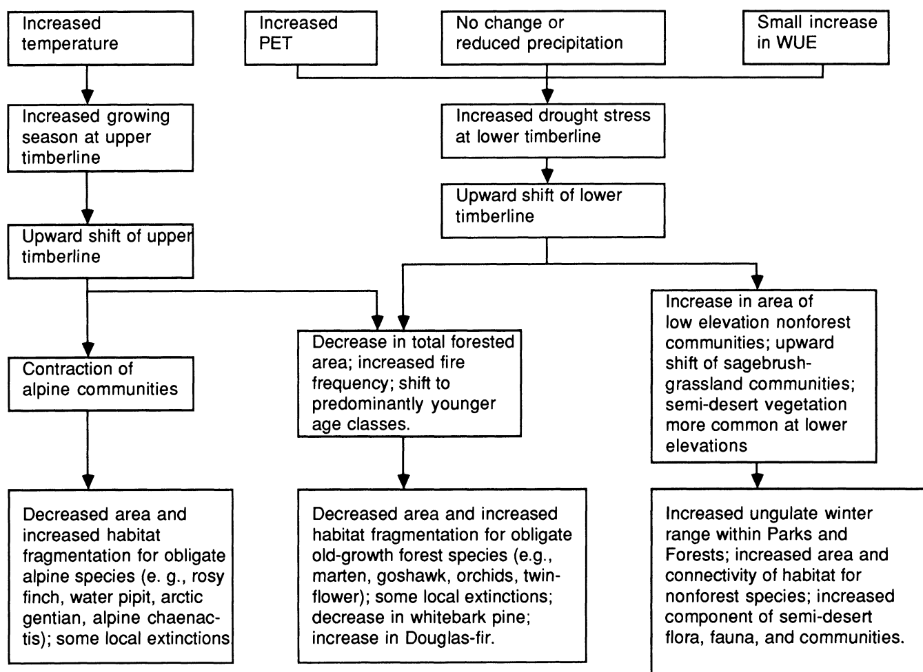
Figure 2. Potential effects on the Greater Yellowstone Ecosystem of a climate that is warmer and drier than the present climate (scenario 1).
