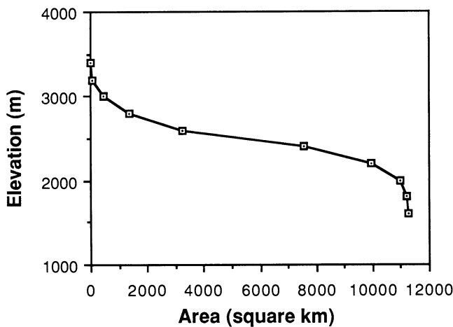
Figure 5. Cumulative area above each elevation zone within Yellowstone National Park and the adjacent mountains along its eastern border. (Data courtesy of the National Park Service.)
