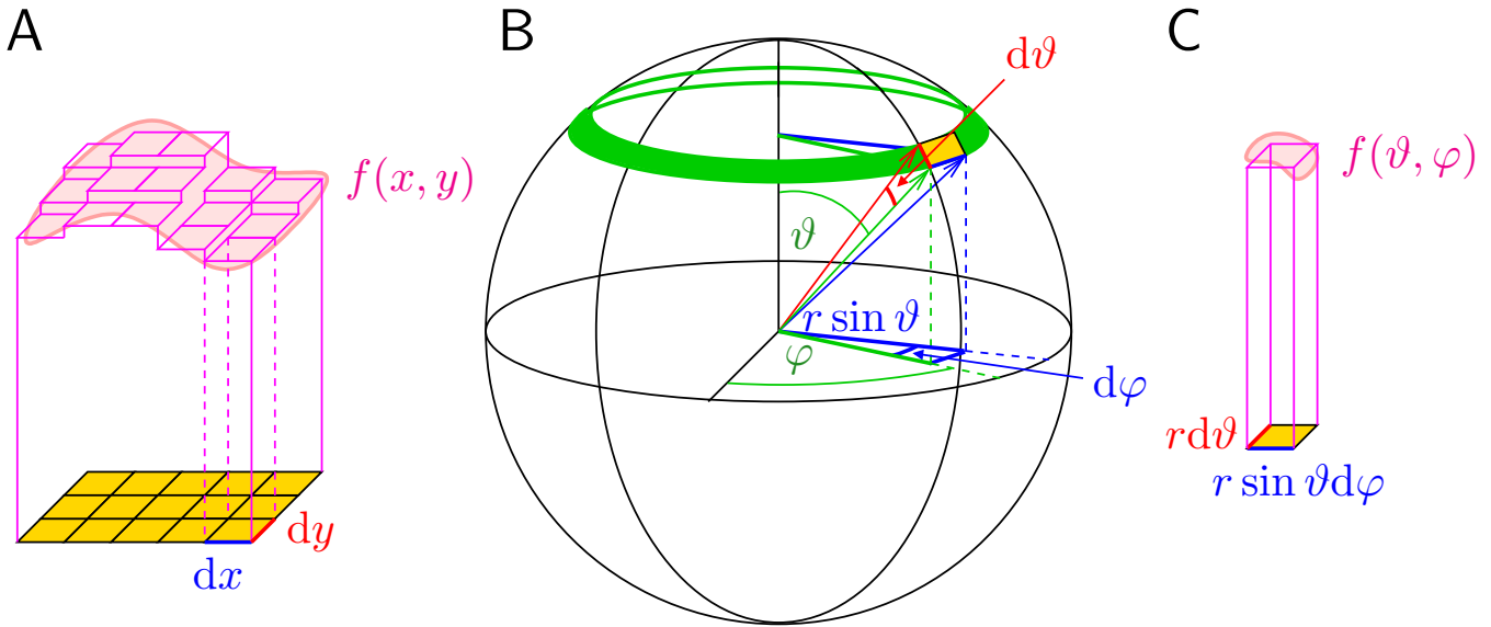
Figure 1.7: Integration in calculating averages. Integration of f(x, y) (A), integration of f(\vartheta, \varphi) , and the volume element f(\vartheta, \varphi)r^2 \sin \vartheta d\vartheta d\varphi (C). Details are described in the text.
