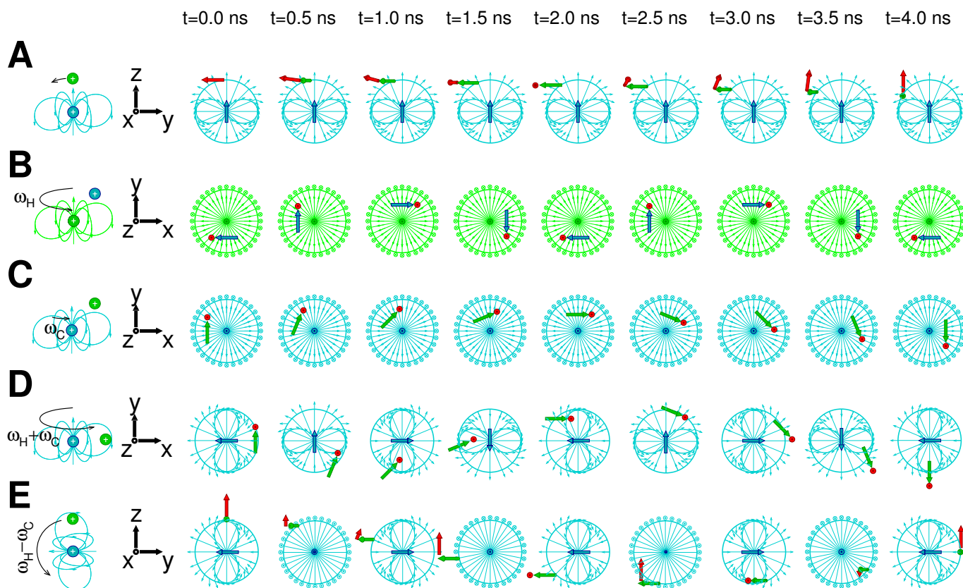
Figure 8.2: Illustration how random molecular motions resonating with five characteristic frequencies affect \vec{\mu}_1 = \vec{\mu}_C in the CH bond in a 500 MHz spectrometer ( \vec{B}_0 = 11.75 T). The first diagram in each row shows positions of the nuclei ( ^{13}\text{C} in green, ^1\text{H} in cyan), the second diagram shows orientation of the coordinate frame, the following diagrams are snapshots of the orientations of magnetic moments shown as arrows ( ^{13}\text{C} in green, ^1\text{H} in cyan) in a magnetic field of the neighbour (shown as force lines). The red arrow indicates the direction of the change of the orientation of the influenced magnetic moment, but the actual change is very small (not observable in the pictures) in the short depicted period of 4 ns. The molecule is assumed to rotate with a constant frequency for 4 ns. A, \vec{\mu}_1 = \vec{\mu}_C oriented horizontally, \vec{\mu}_2 = \vec{\mu}_H oriented vertically, ^{13}\text{C} in the yz plane, ^1\text{H} in the center of the coordinate system. Rotation at any frequency about a horizontal axis varies precession frequency of \vec{\mu}_C about \vec{B}_0 and results in the loss of coherence of ^{13}\text{C} . B, \vec{\mu}_H oriented horizontally, \vec{\mu}_C oriented vertically, ^1\text{H} above the xy plane, ^{13}\text{C} in the center of the coordinate system. Rotation at \omega_H about a horizontal axis pulls \vec{\mu}_H up (red arrow pointing up in the given coordinate frame) in the magnetic fields of \vec{\mu}_C . This reorientation of \vec{\mu}_H (observed only at time much longer than the depicted period of 4 ns) influences the effect of the J -coupling. C, \vec{\mu}_C oriented horizontally, \vec{\mu}_H oriented vertically, ^{13}\text{C} above the xy plane, ^1\text{H} in the center of the coordinate system. Rotation at \omega_C about a horizontal axis pulls \vec{\mu}_C up (red arrow pointing up in the given coordinate frame) in the magnetic fields of \vec{\mu}_H . D, \vec{\mu}_C oriented horizontally, \vec{\mu}_H oriented horizontally, ^{13}\text{C} in the xy plane, ^1\text{H} in the center of the coordinate system. Rotation at \omega_H + \omega_C about a horizontal axis pulls \vec{\mu}_C up (red arrow pointing up in the given coordinate frame) in the magnetic fields of \vec{\mu}_H . E, \vec{\mu}_C oriented horizontally, \vec{\mu}_H oriented horizontally, ^{13}\text{C} in the yz plane, ^1\text{H} in the center of the coordinate system. Rotation at \omega_H - \omega_C about a horizontal axis pulls \mu_C up (red arrow pointing mostly up in the given coordinate frame) in the magnetic fields of \mu_H . The reorientation of \mu_C in Panels C–E (observed only at time much longer than the depicted period of 4 ns) contributes to the return of the distribution of the ^{13}\text{C} magnetic moments to the thermal equilibrium.
