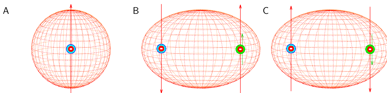
Figure 10.1: J -coupling. A, probability of finding an electron in the hydrogen atom at particular coordinates is described by the probability density \rho . The probability density described by the orbital 1s (depicted as a sphere) has non-zero value at the position of the nucleus (shown in cyan). Therefore, there is a non-zero probability of finding electron (red circle) exactly at the site of the nucleus. The field produced at the site of the nucleus by the electron's magnetic moment (red arrow) does not depend on the orientation of the atom if the positions of the nucleus and electron coincide. Therefore, the interaction of the nucleus with the electron is not averaged to zero if the atom rotates isotropically. B and C, the probability density described by the sigma orbitals (depicted as an ellipsoid) in molecules has also non-zero values at the sites of nuclei. The spin state of the electrons in the bonding sigma orbital is a superposition of the |\alpha\rangle \otimes |\beta\rangle and |\beta\rangle \otimes |\alpha\rangle eigenstates (indicated by the opposite direction of the red arrows), perturbed by the magnetic moment of the nuclei. The parallel orientations of magnetic moments is energetically favorable for a nucleus and an electron sharing its position.
