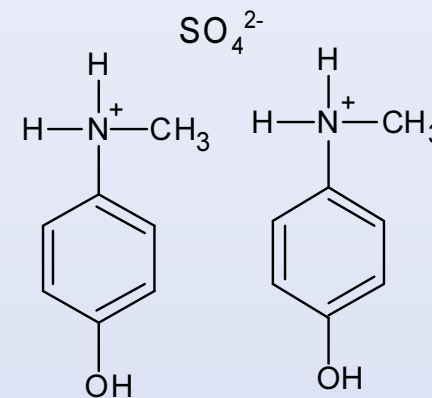
metol
