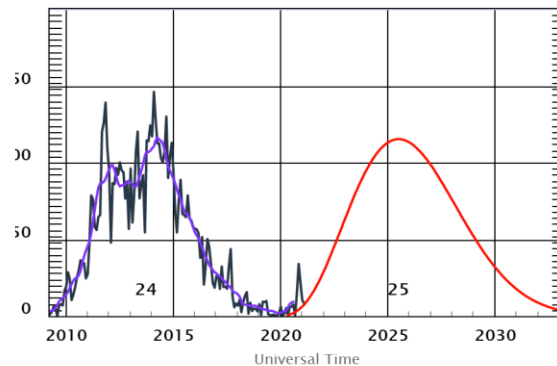
ISES Solar Cycle Sunspot Number Progression
