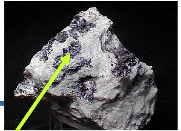
diaspor – \text{AlO}(\text{OH})
