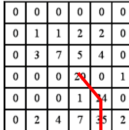
Flow accumulation
