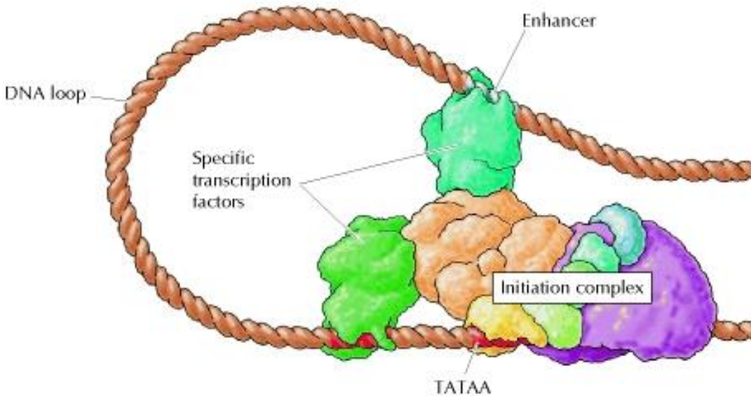
Figure 6.22 DNA looping
