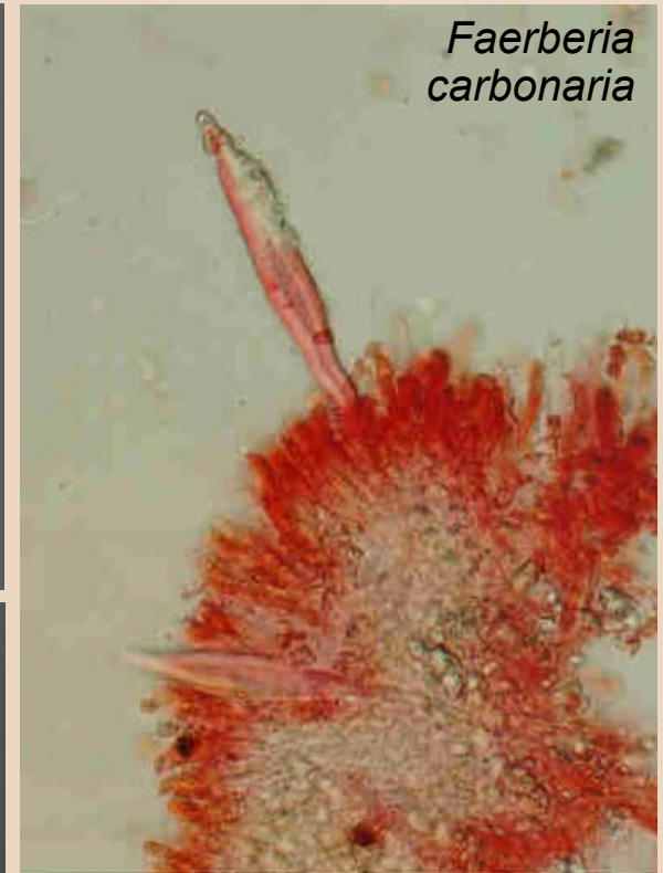
Figure 6.20: Calcium oxalate crystals at the apex and in the wall of Inocybe -cystidia (arrows). The region of the transperietal excretion is metachromatic in Inocybe asterospora , (stippled regions); in many species it is not. – I. fuscidula original photograph; I. asterospora from Waterkeyn, Bennis & Monniez 1992.
