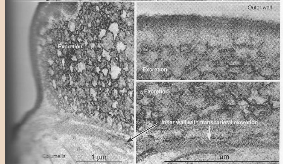
Figure 6.17: The apical swelling of the halocystidia of Resinicium bicolor accumulates an excretion beneath the columella, a unique structure for cystidia.
