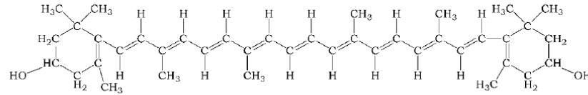
Lutein
