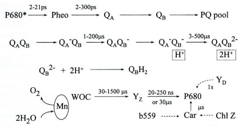
Fig. 2. Diagram showing the main kinetics of the main pathway of electrons through the PS II reaction center. Y D (D2 Tyr161), Chlorophyll Z (Chl Z) and Cytochrome b 559 (b 559 ) are alternate electron donors under certain conditions. See also Figure 1.
