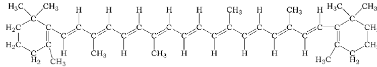
\beta -carotene
