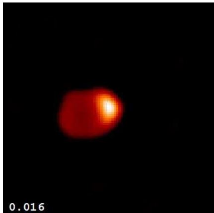
\beta Persei
