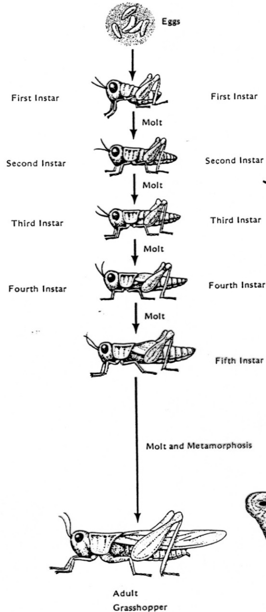
HEMIMETABOLOUS DEVELOPMENT
