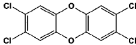
2,3,7,8-TCDD
