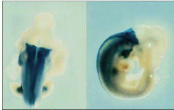
dorsal view
