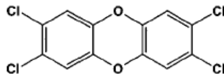
2,3,7,8-TCDD
