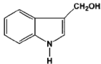
I3C
