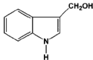
I3C
