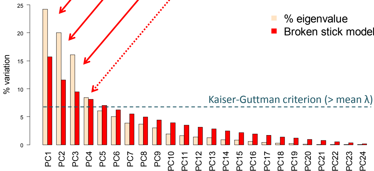
Screeplot
