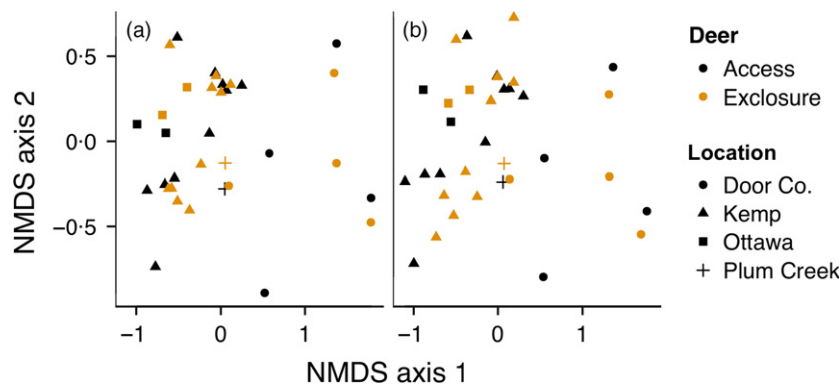
Fig. 5. Ordinations of environmental conditions across all deer-access and exclusion plots. To depict the understorey environment for tree saplings (a), we conducted non-metric multidimensional scaling (NMDS) of 17 plot-level abiotic (soil surface horizons, chemistry, texture and compaction) and biotic (earthworm invasion rank, CWD and basal area of trees) environmental variables. Stress = 0.14. To depict the groundlayer environment for herbs, shrubs and tree seedlings, we generated an NMDS of 20 plot-level environmental variables (b), which included all variables from (a) with the addition of openness, the basal area of hardwood saplings and the basal area of conifer saplings. Stress = 0.12. Based on results of PERMANOVA, NMDS scores of the groundlayer environment differed between exclusion and deer-access plots ( P \leq 0.05 ). [Colour figure can be viewed at wileyonlinelibrary.com ]
