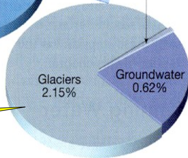
Nonocean Component (% of total hydrosphere)
