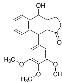
podofyllotoxin (cytostatikum)
