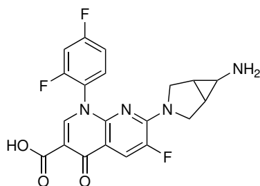
trovafloxacin (antibiotikum)
