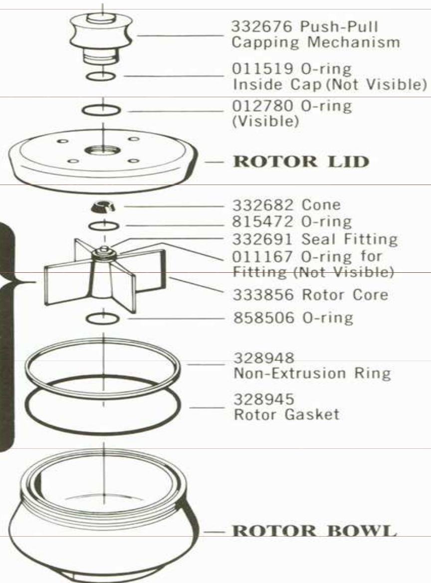
B-29 Type Core
