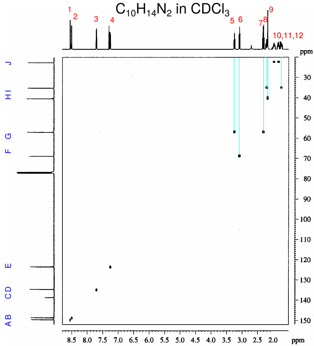
^{13}C, ^1H HSQC
