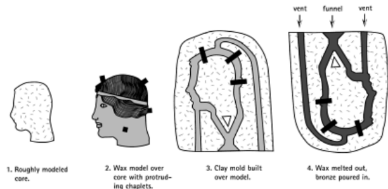
Hollow Lost-Wax Casting: The Direct Method Drawing © Seán Hemingway
