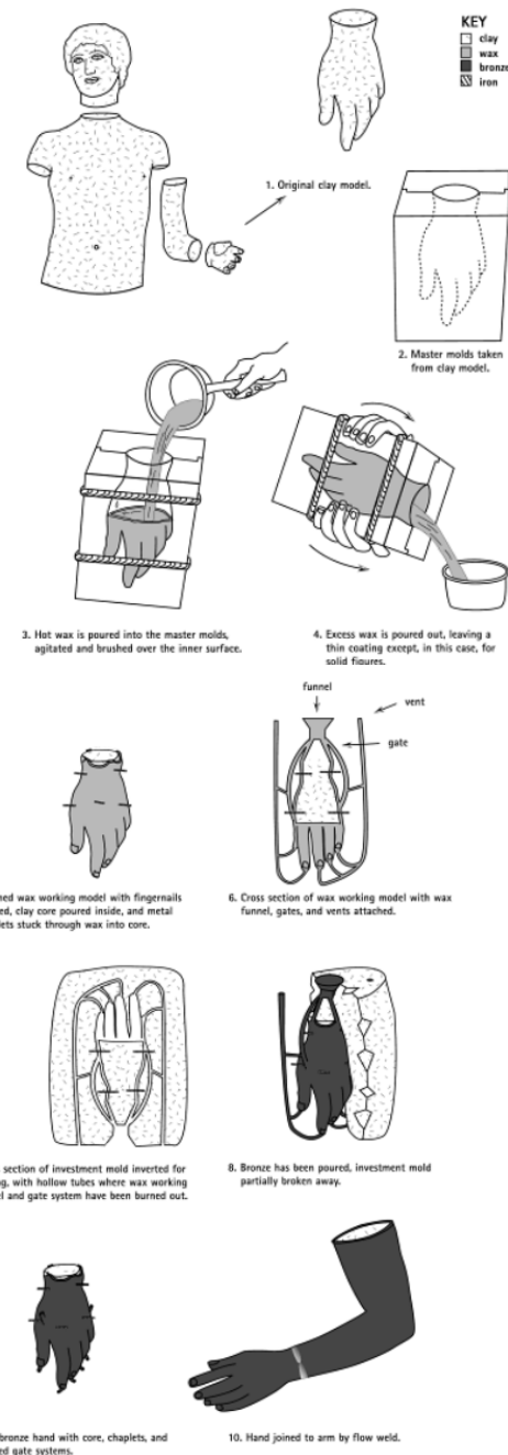
Hollow Lost-Wax Casting: The Indirect Method Drawing © Seán Hemingway
