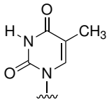
thymin
