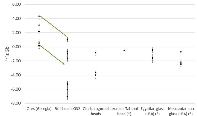
Fig. 1. Sb isotopic composition of Caucasian stibnite from the Racha-Lechkumi region and Sb metal beads from Brili and Chalipiragorebi, compared to previously analysed Egyptian and Mesopotamian Late Bronze Age glasses (Degryse et al., 2015). The arrows show the 3-epsilon correction for fractionation between the unprocessed ores and the archaeological artefacts.
