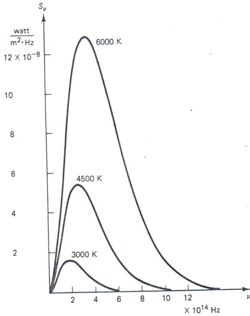
Fig. 3.5 Spectral emittance as a function of frequency according to Planck's law, at three different temperatures.
