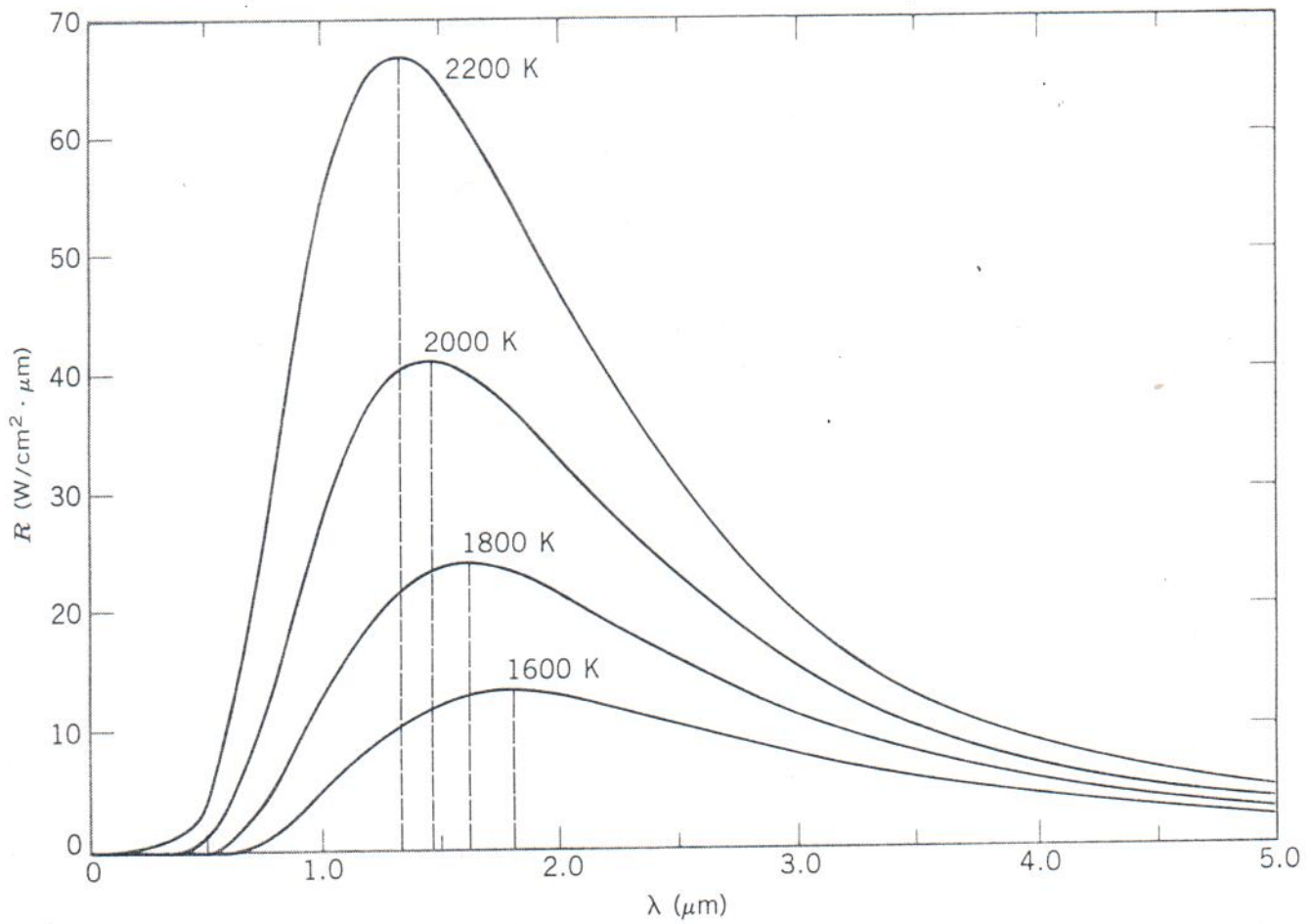
Figure 3 Spectral radiancy curves for cavity radiation at four selected temperatures. Note that as the temperature increases, the wavelength of the maximum spectral radiancy shifts to lower values.
